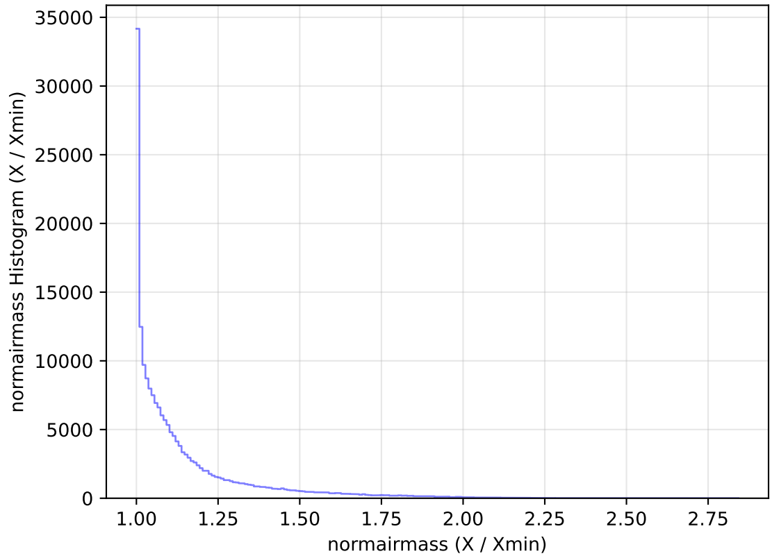
internal_u_expt38_nscale0.9v3.4_10yrs WFD g band: normairmass Histogram
