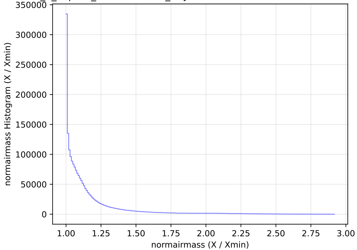
internal_u_expt38_nscale0.9v3.4_10yrs WFD all bands: normairmass Histogram
