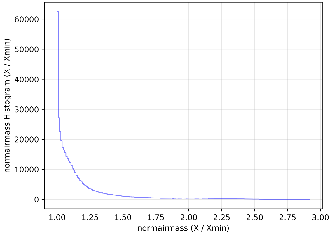
internal_u_expt38_nscale0.9v3.4_10yrs All sky z band: normairmass Histogram
