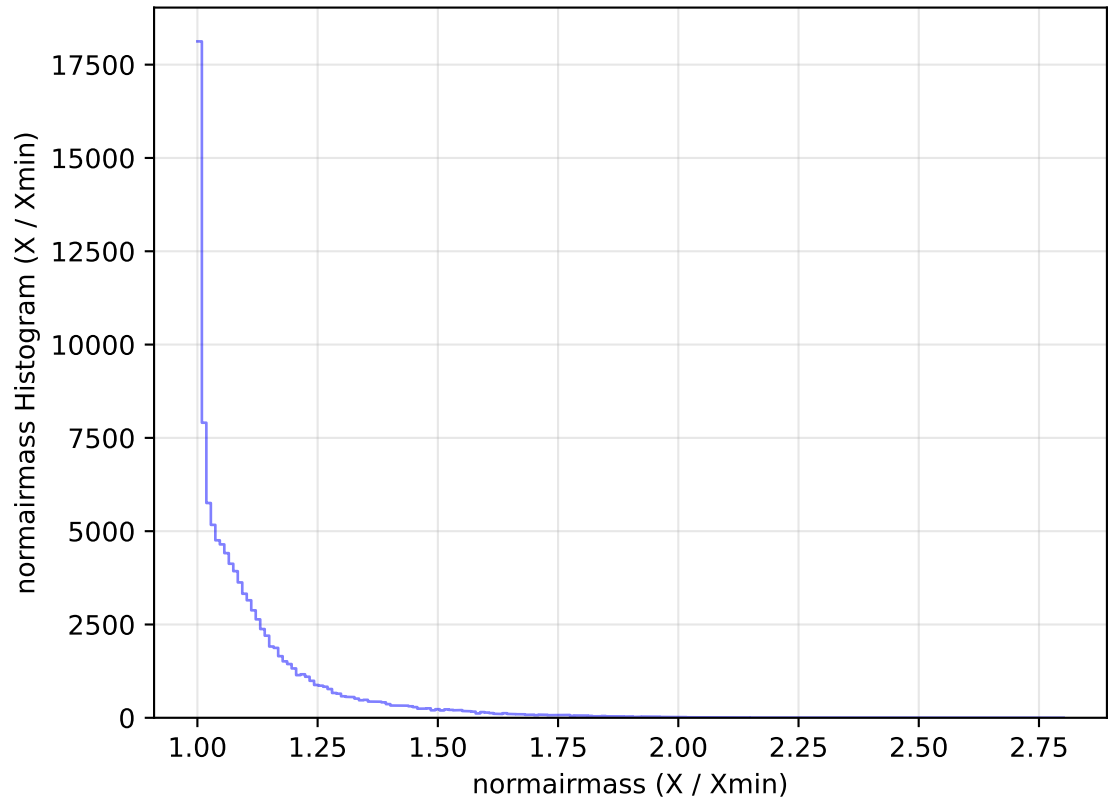
internal_u_expt38_nscale0.9v3.4_10yrs All sky u band: normairmass Histogram
