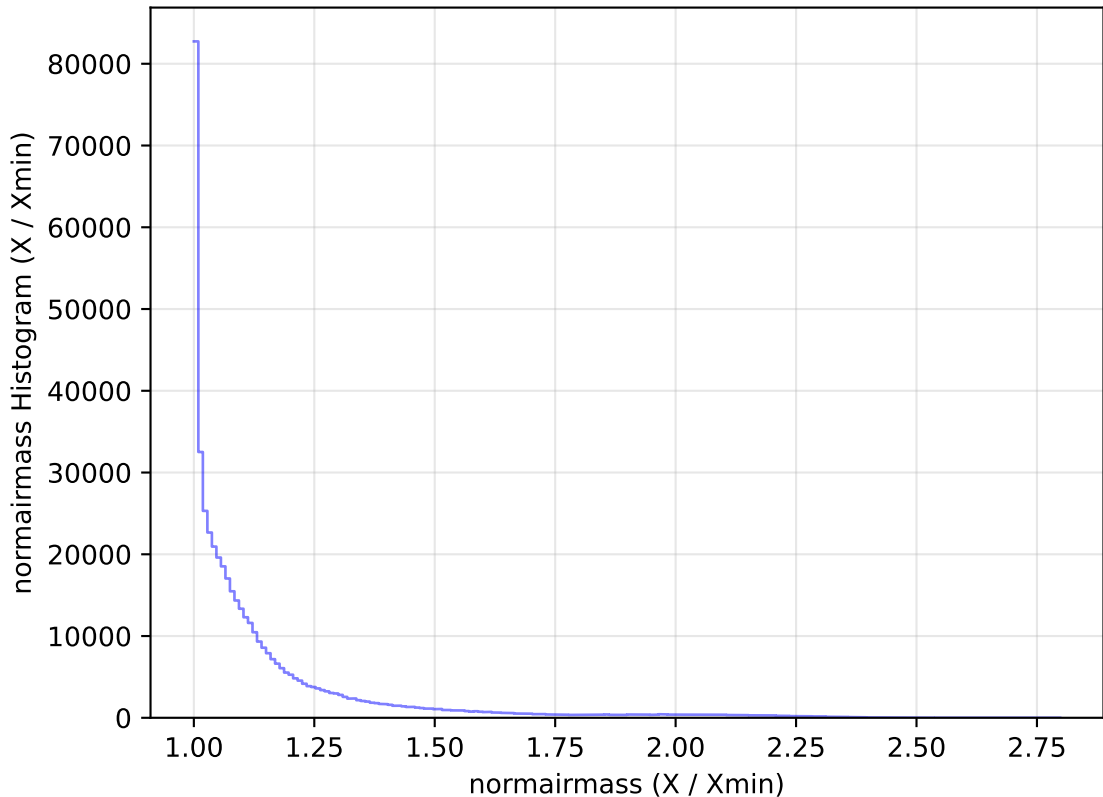
internal_u_expt38_nscale0.9v3.4_10yrs All sky r band: normairmass Histogram
