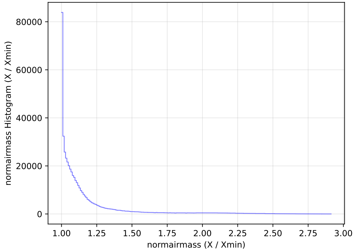
internal_u_expt38_nscale0.9v3.4_10yrs All sky i band: normairmass Histogram
