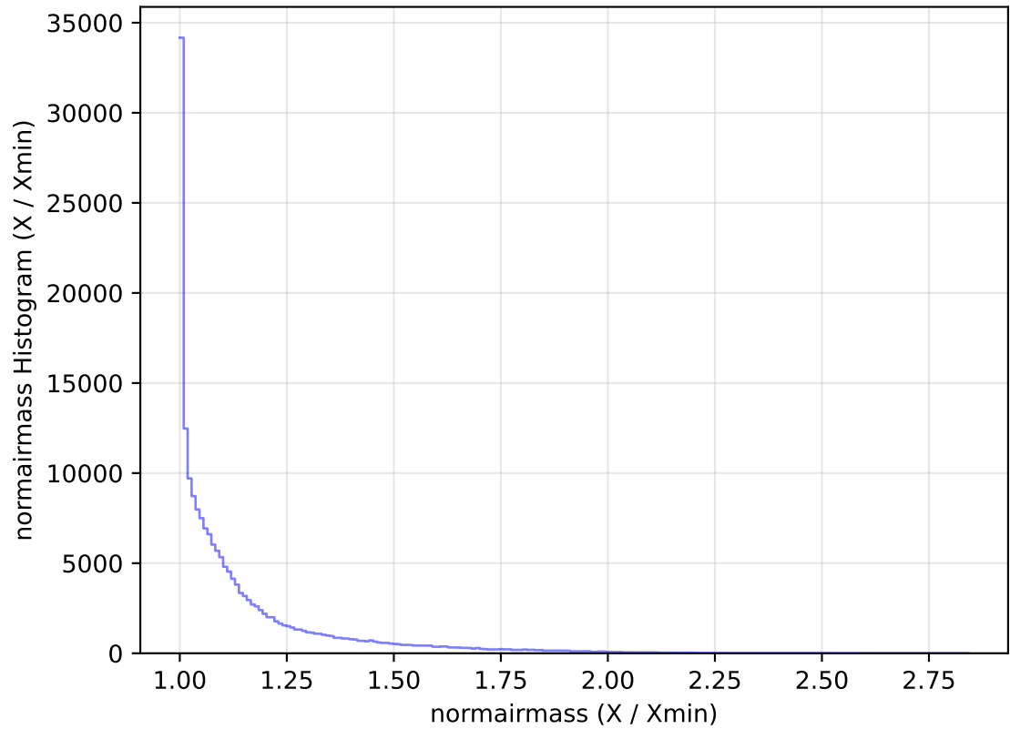
internal_u_expt38_nscale0.9v3.4_10yrs All sky g band: normairmass Histogram
