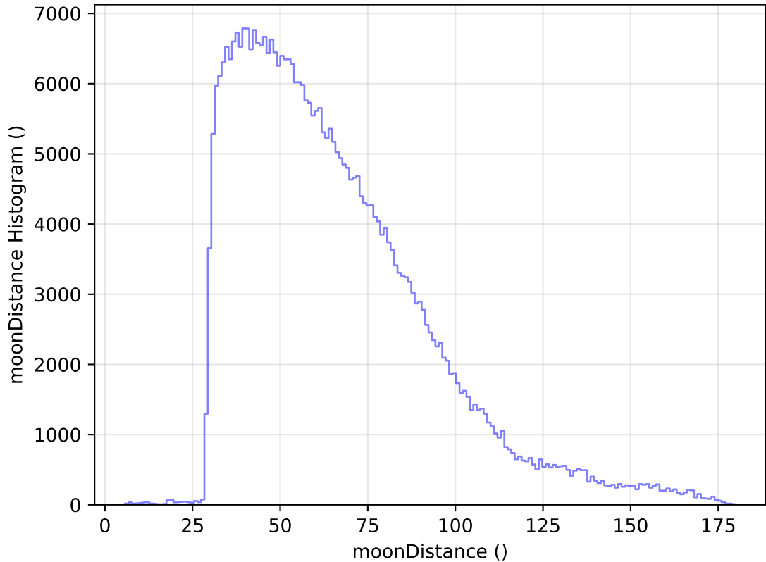
internal_u_expt38_nscale0.9v3.4_10yrs WFD y band: moonDistance Histogram
