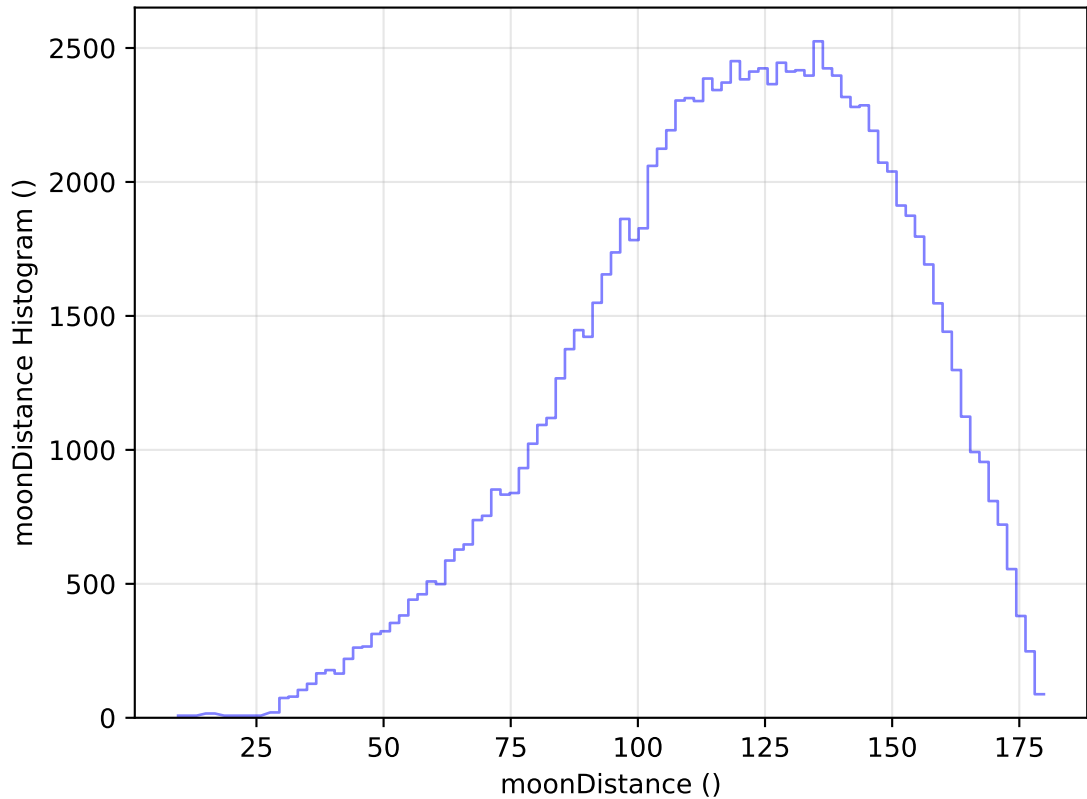
internal_u_expt38_nscale0.9v3.4_10yrs WFD u band: moonDistance Histogram
