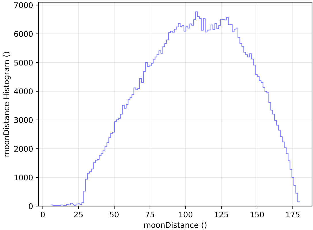
internal_u_expt38_nscale0.9v3.4_10yrs WFD r band: moonDistance Histogram
