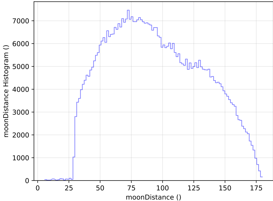
internal_u_expt38_nscale0.9v3.4_10yrs WFD i band: moonDistance Histogram
