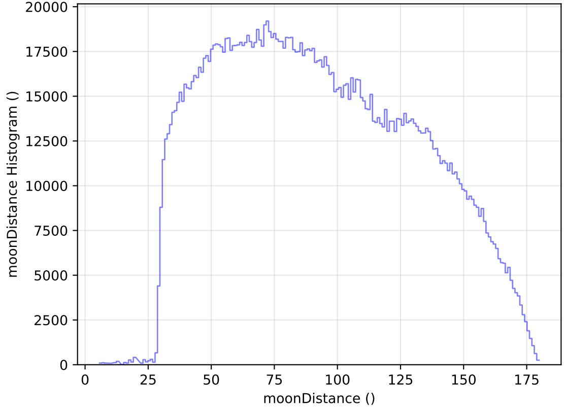
internal_u_expt38_nscale0.9v3.4_10yrs WFD all bands: moonDistance Histogram
