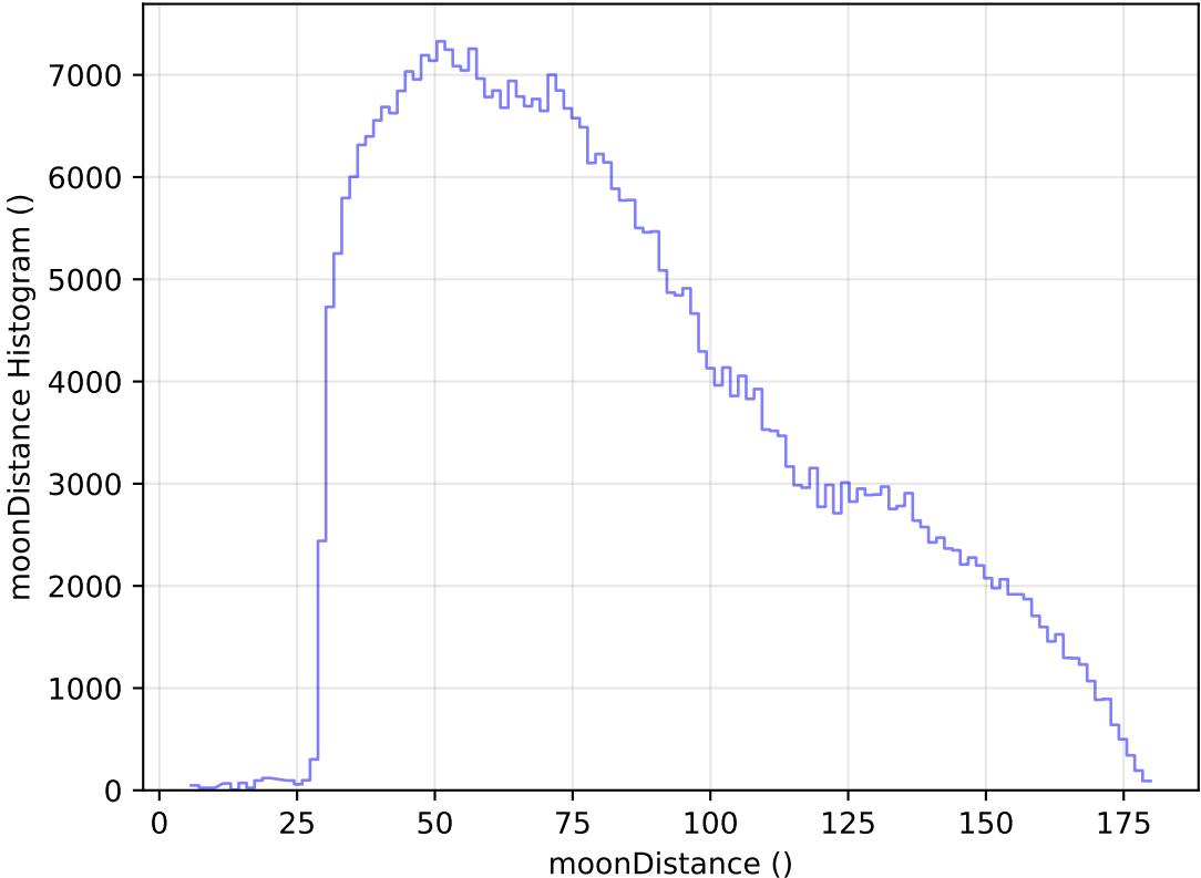
internal_u_expt38_nscale0.9v3.4_10yrs All sky z band: moonDistance Histogram
