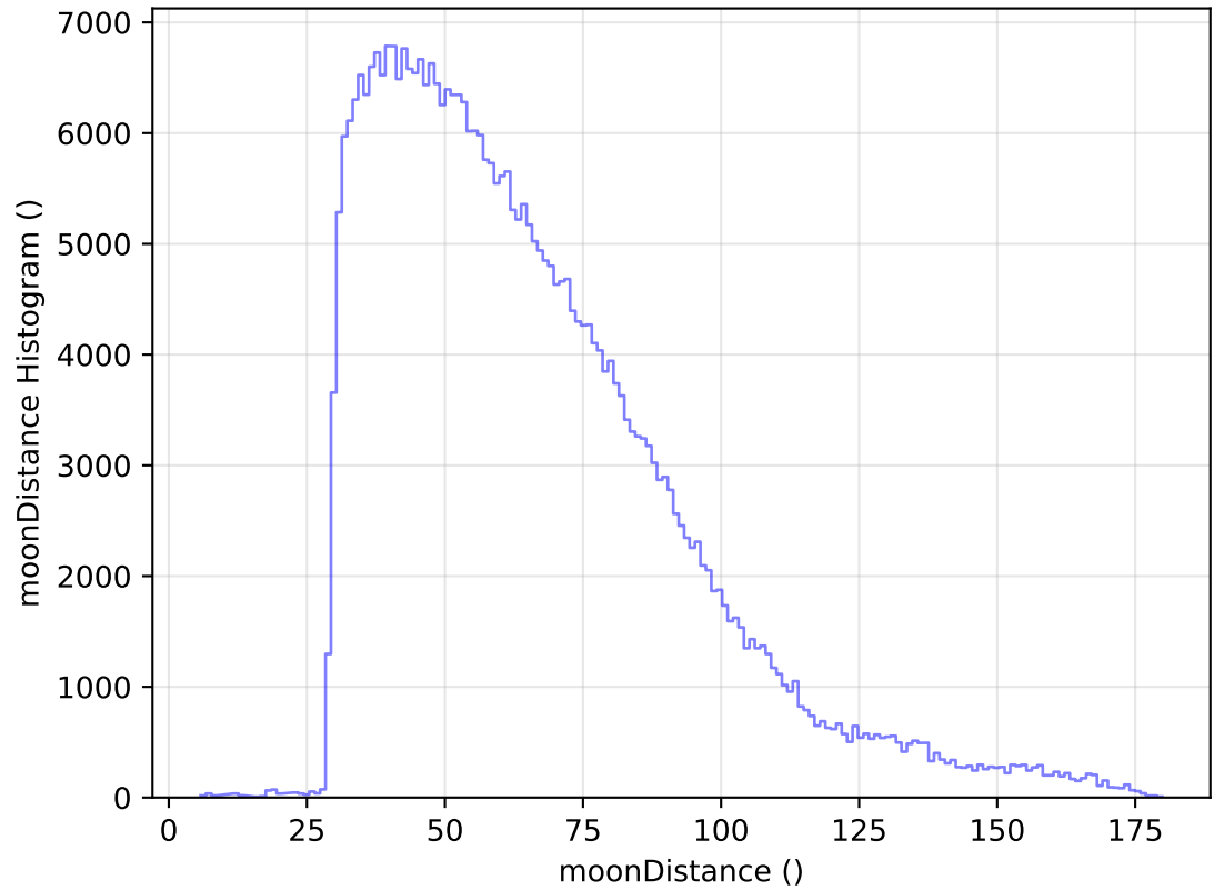
internal_u_expt38_nscale0.9v3.4_10yrs All sky y band: moonDistance Histogram
