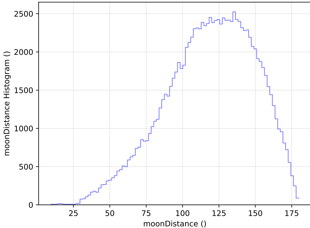
internal_u_expt38_nscale0.9v3.4_10yrs All sky u band: moonDistance Histogram
