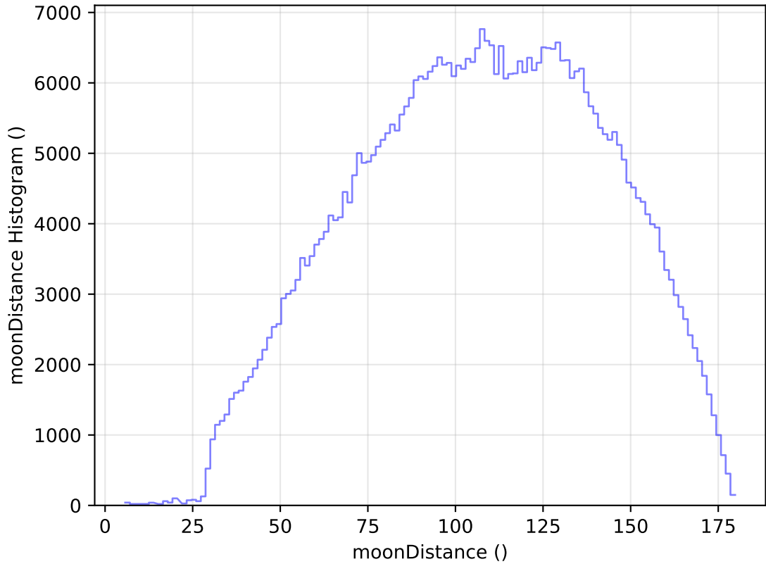
internal_u_expt38_nscale0.9v3.4_10yrs All sky r band: moonDistance Histogram
