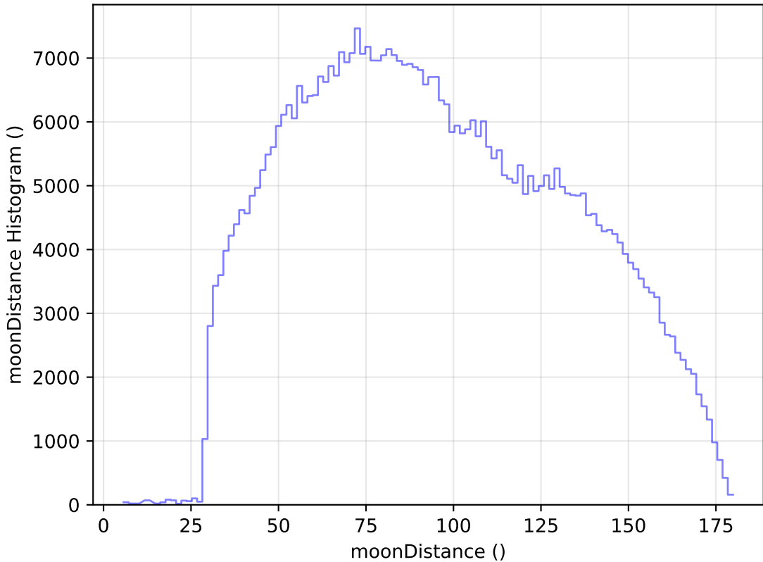
internal_u_expt38_nscale0.9v3.4_10yrs All sky i band: moonDistance Histogram
