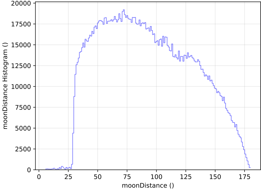
internal_u_expt38_nscale0.9v3.4_10yrs All sky all bands: moonDistance Histogram
