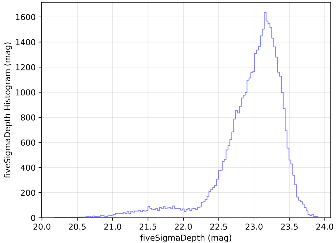
internal_u_expt38_nscale0.9v3.4_10yrs Yr 1 z band: fiveSigmaDepth Histogram
