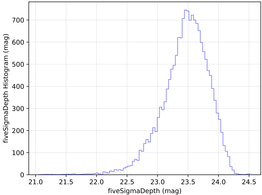
internal_u_expt38_nscale0.9v3.4_10yrs Yr 1 u band: fiveSigmaDepth Histogram
