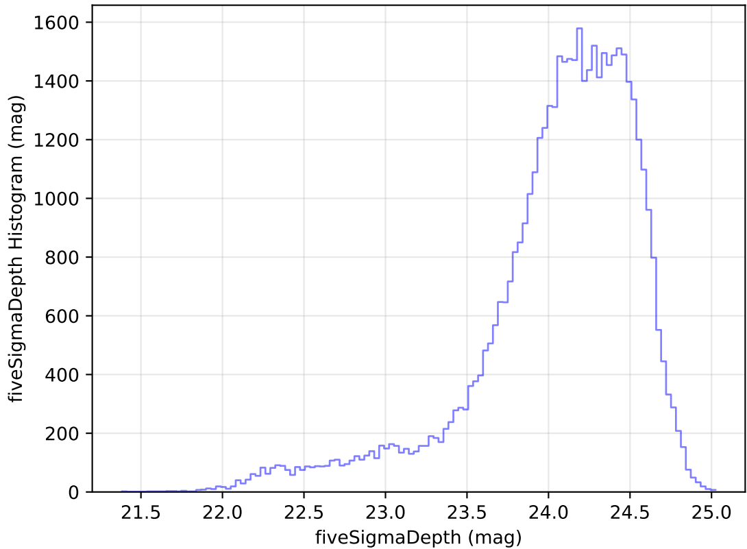
internal_u_expt38_nscale0.9v3.4_10yrs Yr 1 r band: fiveSigmaDepth Histogram
