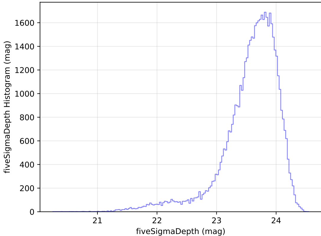
internal_u_expt38_nscale0.9v3.4_10yrs Yr 1 i band: fiveSigmaDepth Histogram
