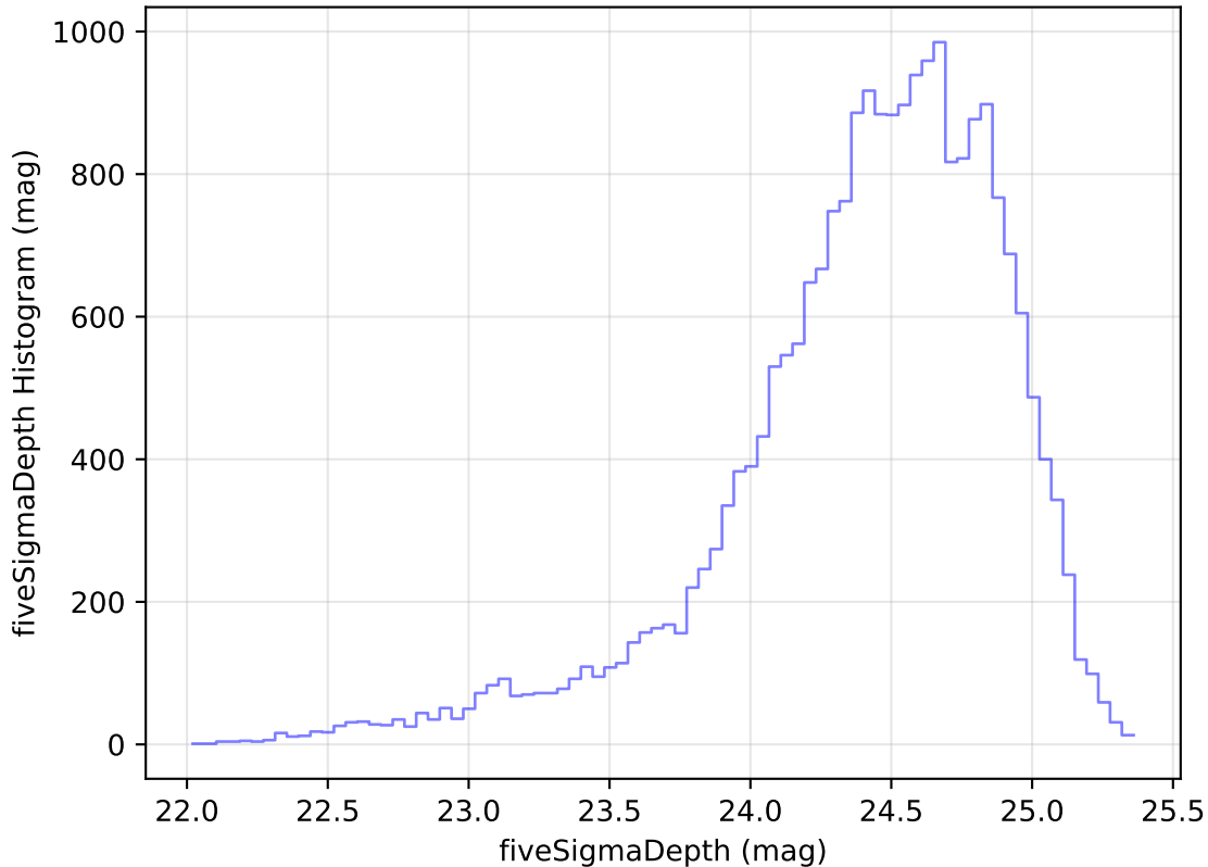
internal_u_expt38_nscale0.9v3.4_10yrs Yr 1 g band: fiveSigmaDepth Histogram
