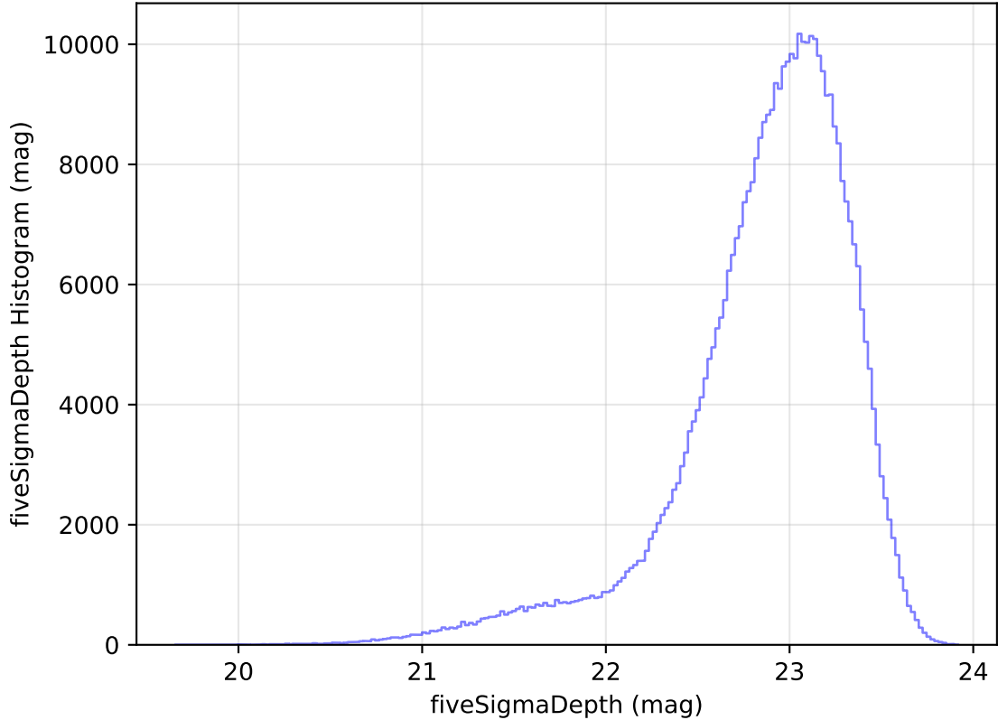
internal_u_expt38_nscale0.9v3.4_10yrs WFD z band: fiveSigmaDepth Histogram
