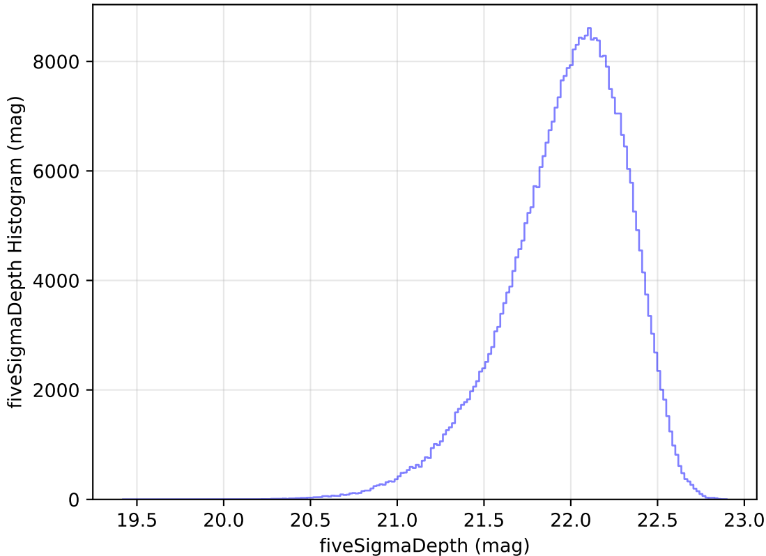
internal_u_expt38_nscale0.9v3.4_10yrs WFD y band: fiveSigmaDepth Histogram
