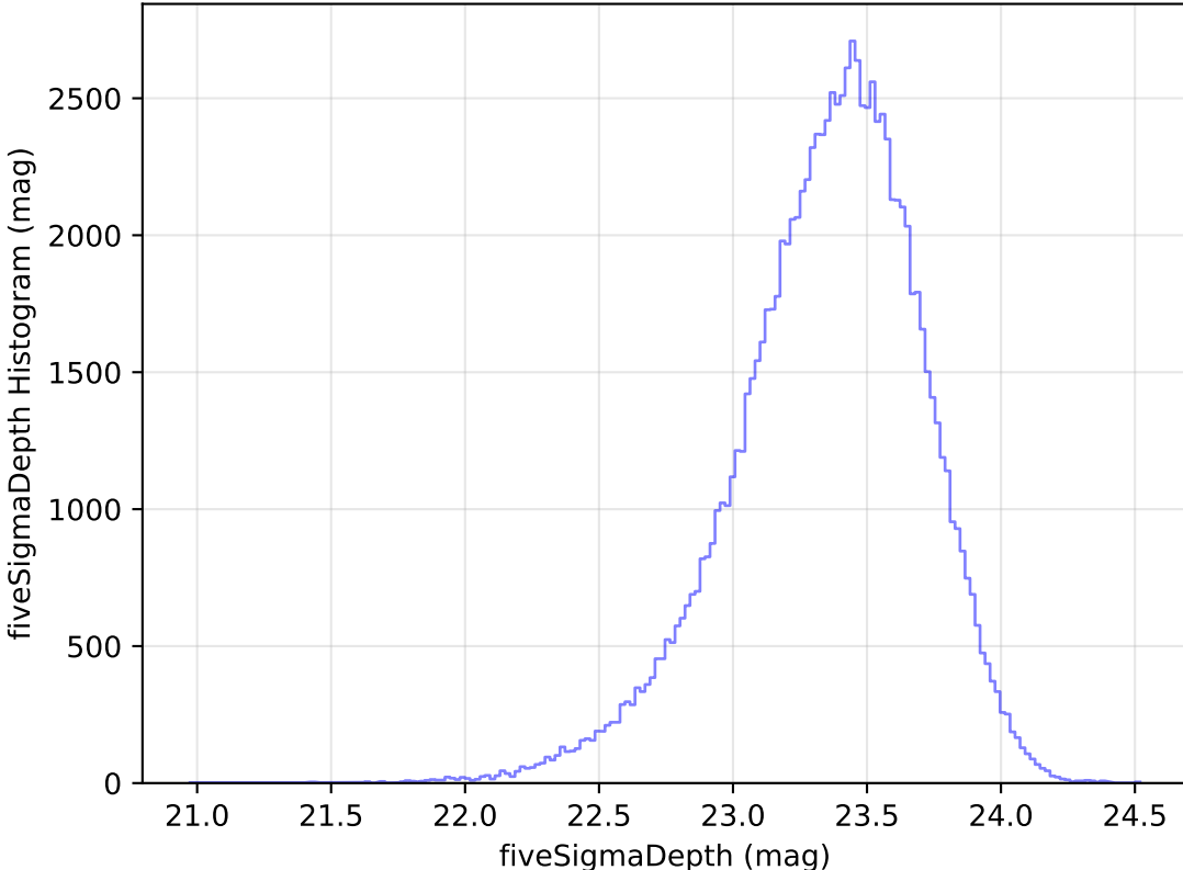
internal_u_expt38_nscale0.9v3.4_10yrs WFD u band: fiveSigmaDepth Histogram
