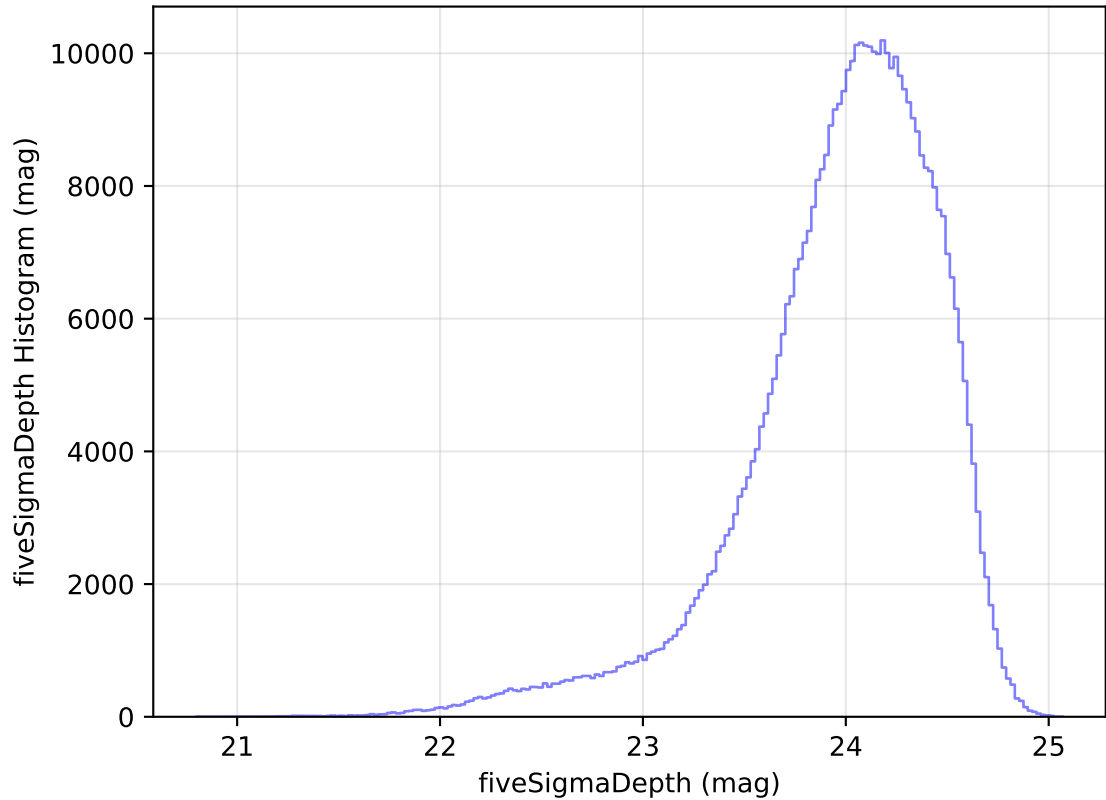
internal_u_expt38_nscale0.9v3.4_10yrs WFD r band: fiveSigmaDepth Histogram
