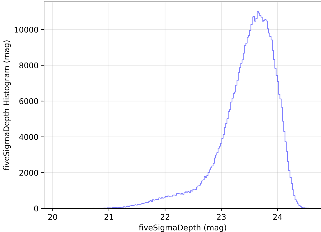
internal_u_expt38_nscale0.9v3.4_10yrs WFD i band: fiveSigmaDepth Histogram
