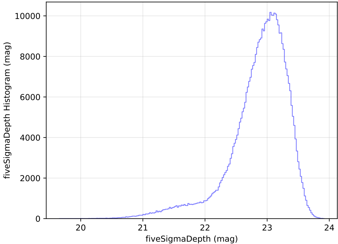
internal_u_expt38_nscale0.9v3.4_10yrs All sky z band: fiveSigmaDepth Histogram
