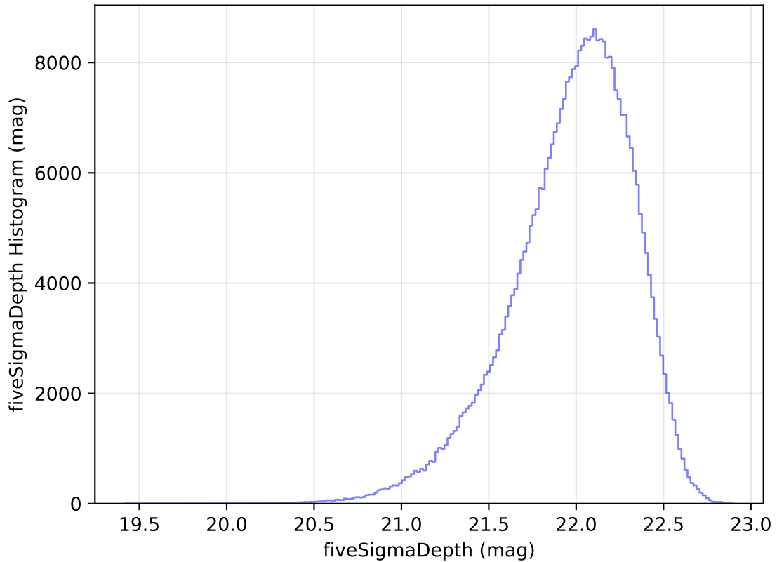
internal_u_expt38_nscale0.9v3.4_10yrs All sky y band: fiveSigmaDepth Histogram
