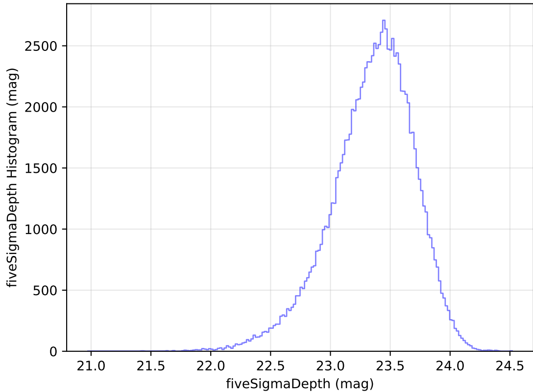
internal_u_expt38_nscale0.9v3.4_10yrs All sky u band: fiveSigmaDepth Histogram
