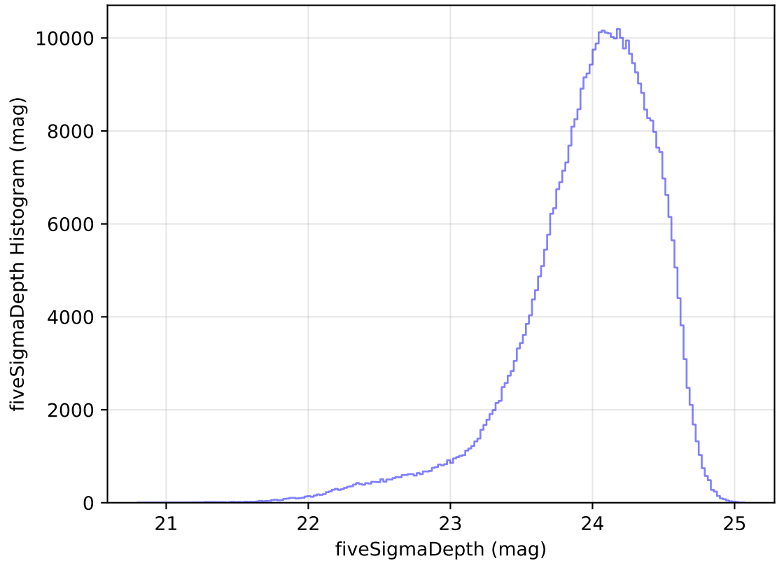
internal_u_expt38_nscale0.9v3.4_10yrs All sky r band: fiveSigmaDepth Histogram
