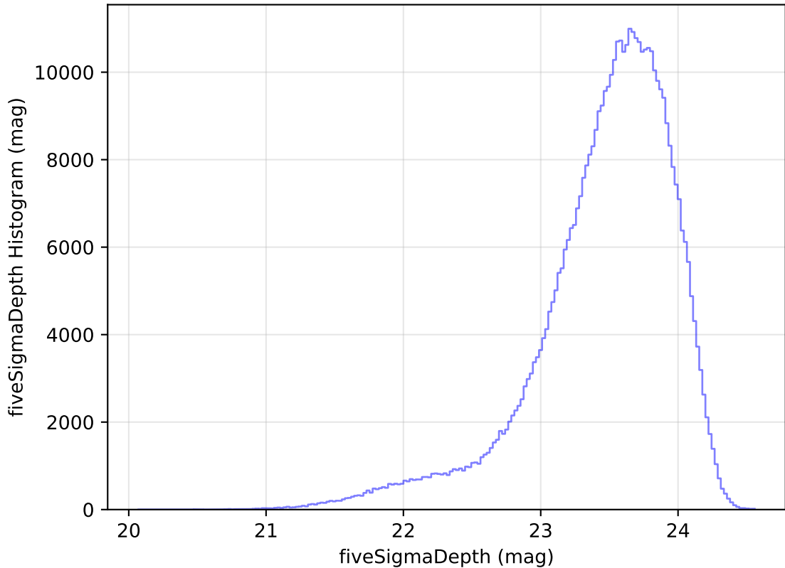
internal_u_expt38_nscale0.9v3.4_10yrs All sky i band: fiveSigmaDepth Histogram
