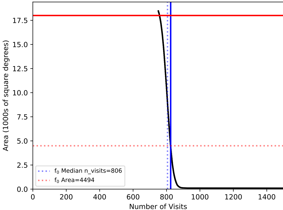
internal_u_expt38_nscale0.9v3.4_10yrs WFD: f0
