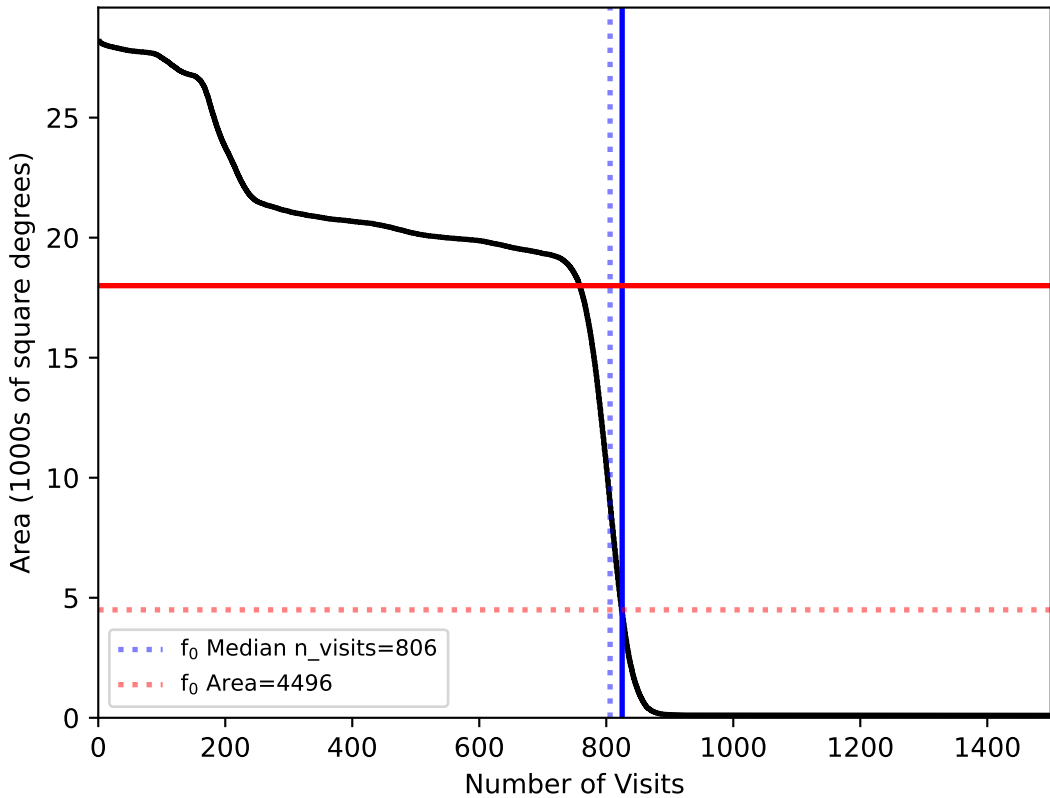
internal_u_expt38_nscale0.9v3.4_10yrs All sky: f0
