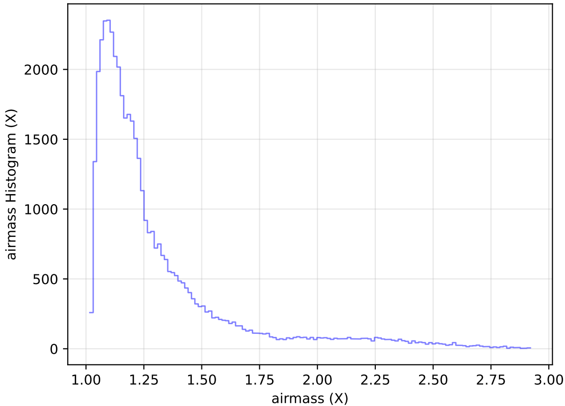
internal_u_expt38_nscale0.9v3.4_10yrs Yr 1 z band: airmass Histogram
