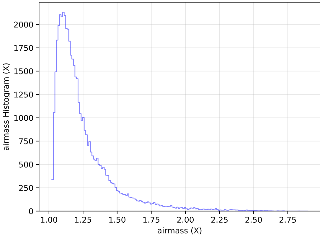
internal_u_expt38_nscale0.9v3.4_10yrs Yr 1 y band: airmass Histogram
