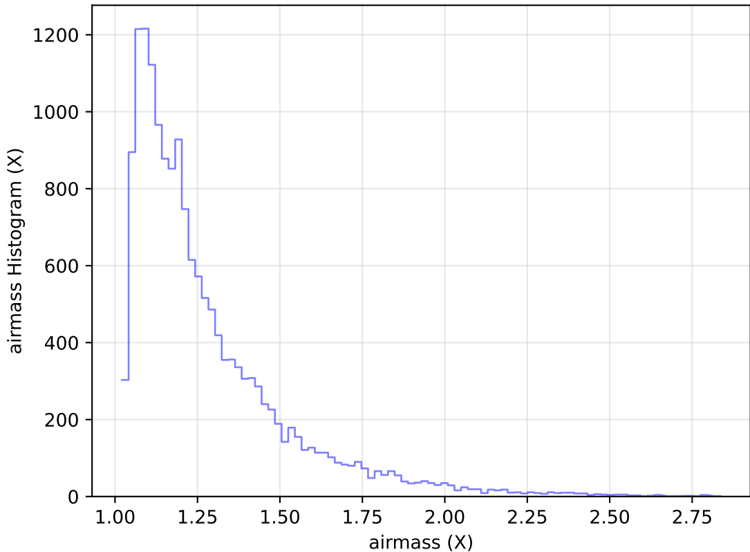
internal_u_expt38_nscale0.9v3.4_10yrs Yr 1 u band: airmass Histogram
