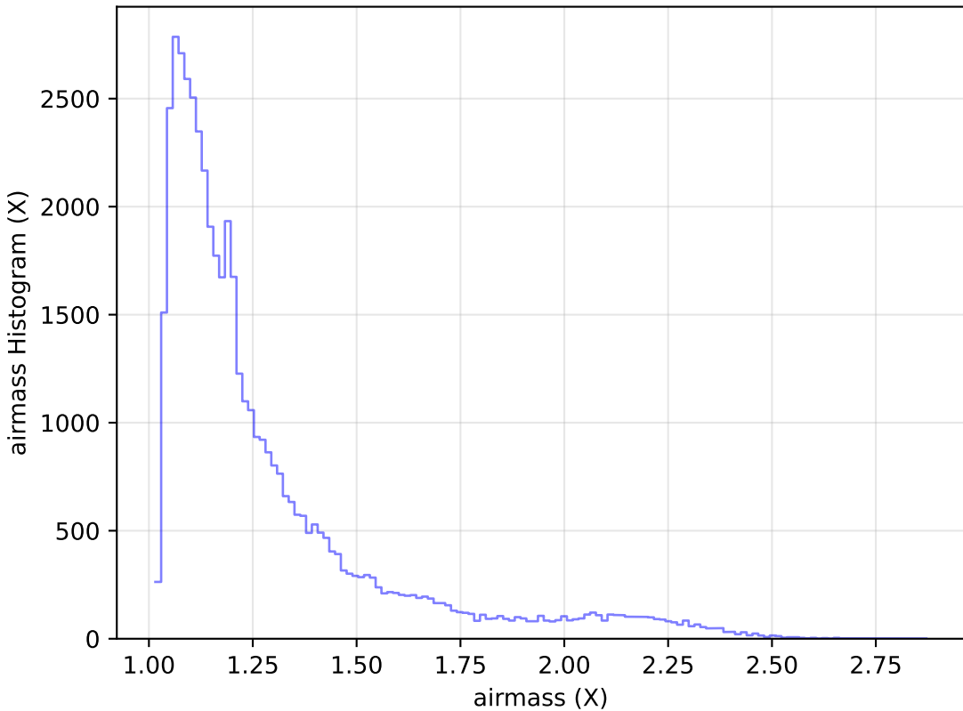
internal_u_expt38_nscale0.9v3.4_10yrs Yr 1 r band: airmass Histogram
