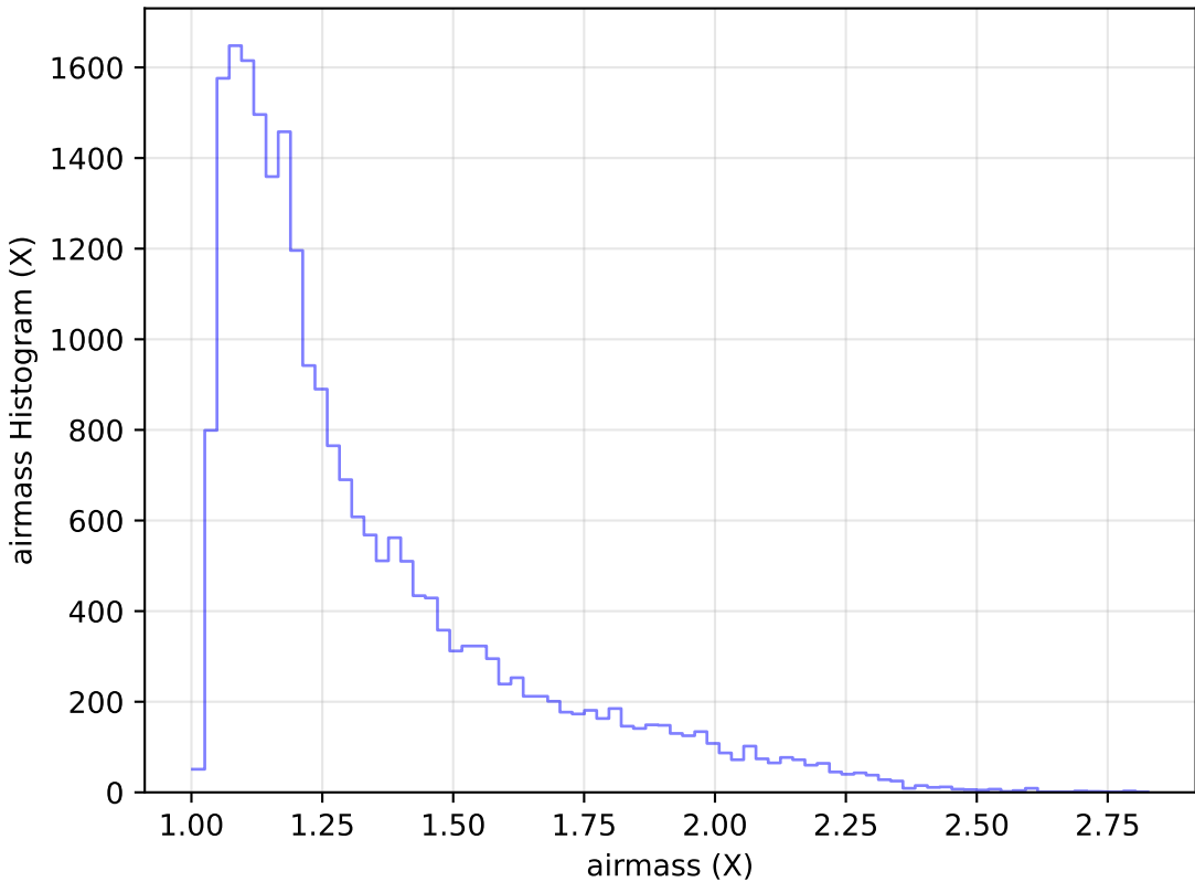
internal_u_expt38_nscale0.9v3.4_10yrs Yr 1 g band: airmass Histogram
