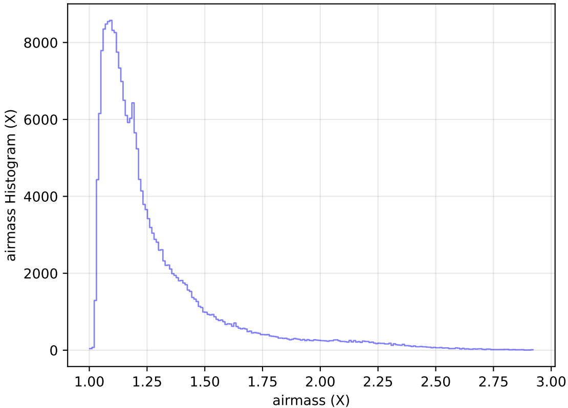
internal_u_expt38_nscale0.9v3.4_10yrs Yr 1 all bands: airmass Histogram
