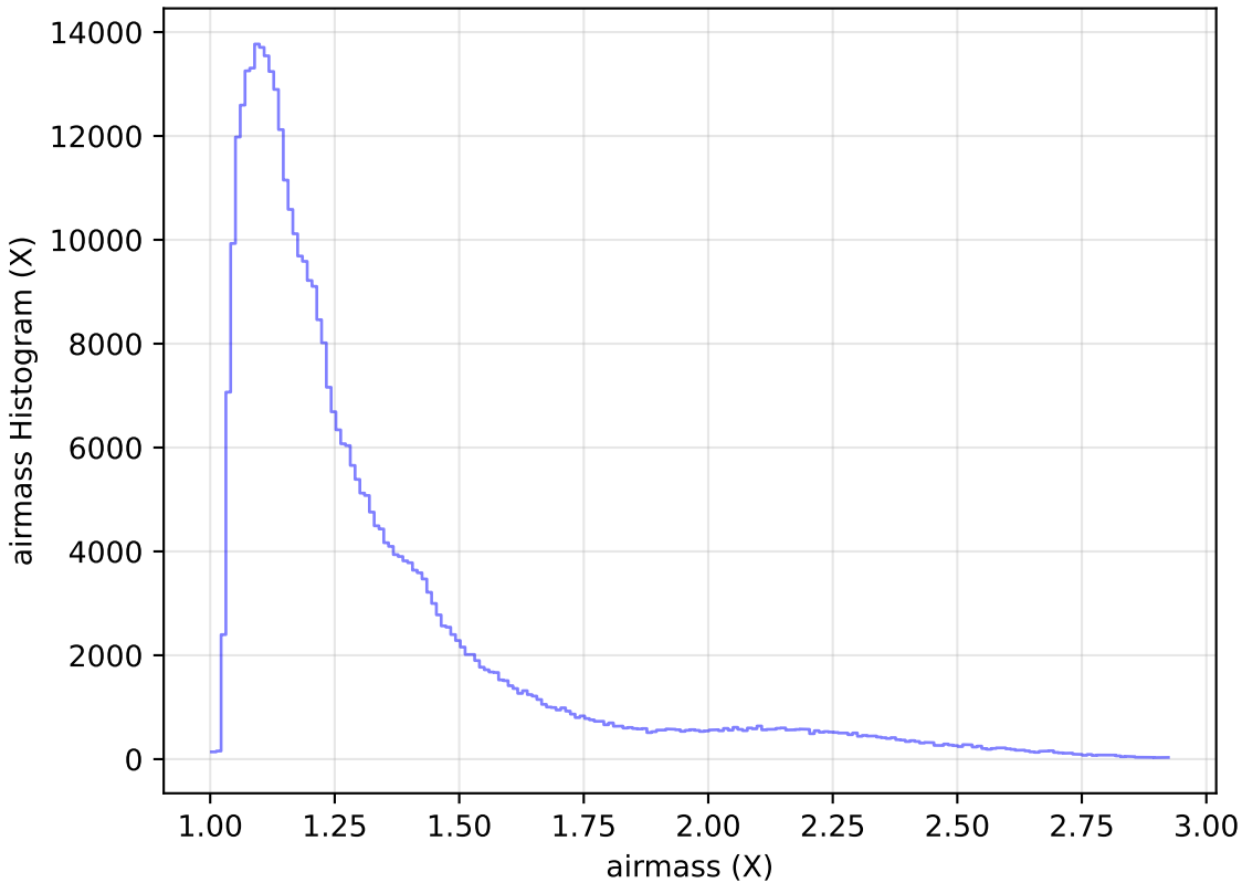
internal_u_expt38_nscale0.9v3.4_10yrs WFD z band: airmass Histogram
