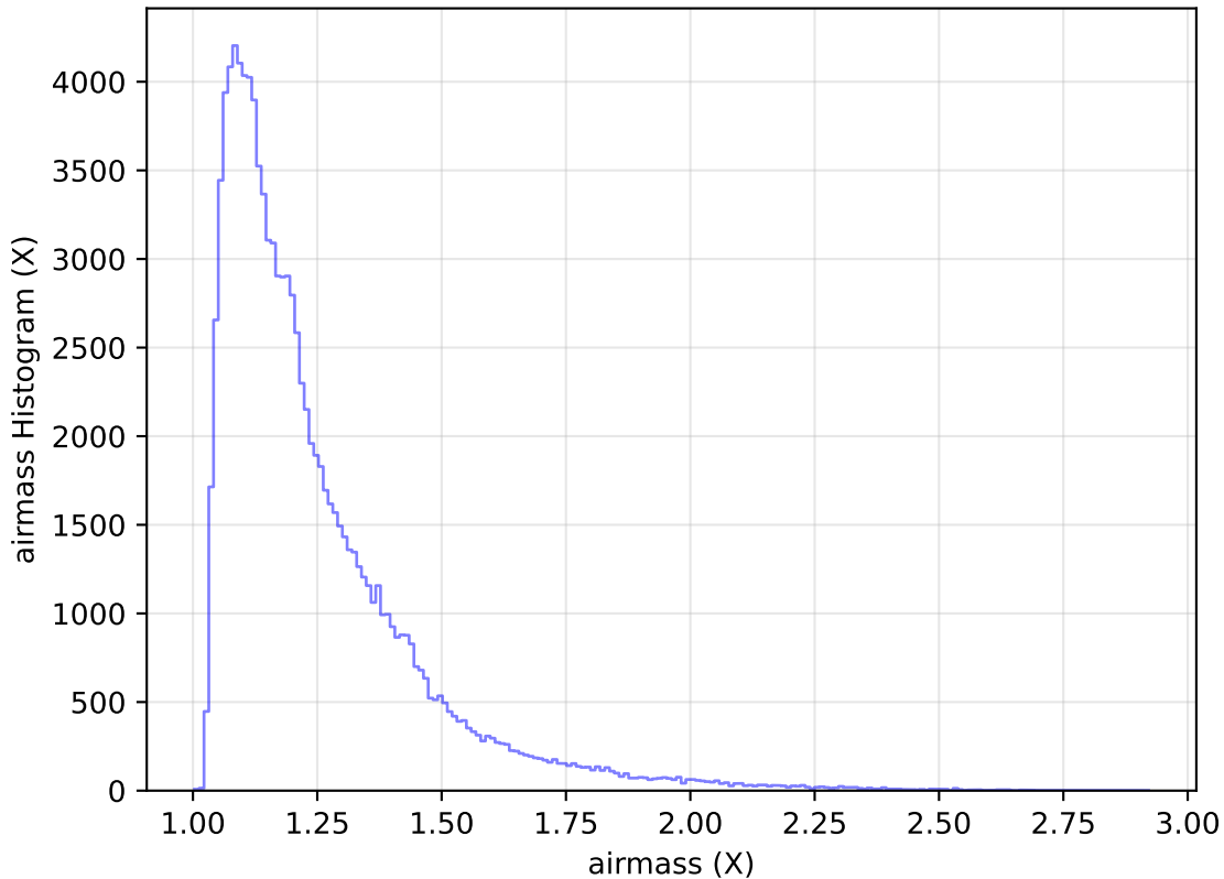
internal_u_expt38_nscale0.9v3.4_10yrs WFD u band: airmass Histogram
