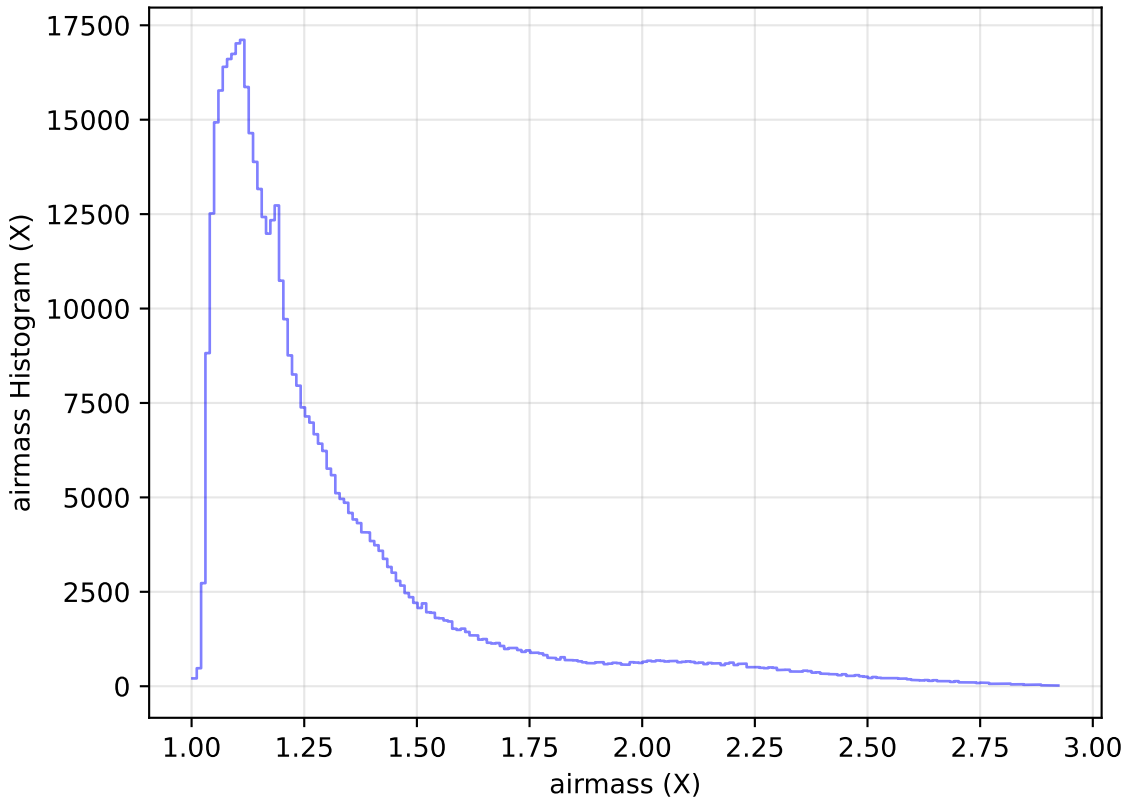
internal_u_expt38_nscale0.9v3.4_10yrs WFD i band: airmass Histogram
