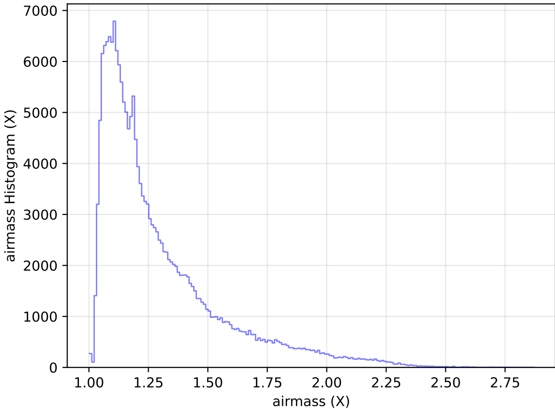
internal_u_expt38_nscale0.9v3.4_10yrs WFD g band: airmass Histogram
