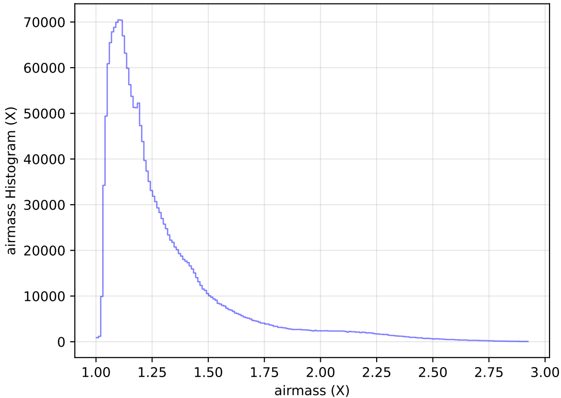
internal_u_expt38_nscale0.9v3.4_10yrs WFD all bands: airmass Histogram
