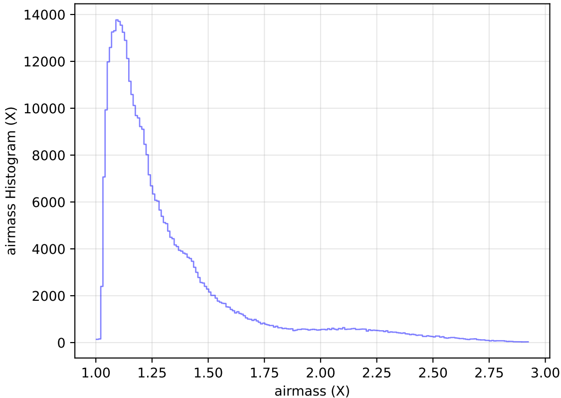
internal_u_expt38_nscale0.9v3.4_10yrs All sky z band: airmass Histogram
