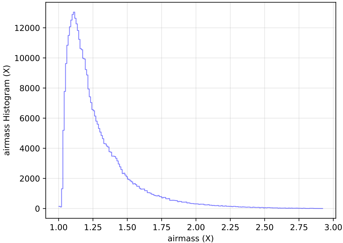
internal_u_expt38_nscale0.9v3.4_10yrs All sky y band: airmass Histogram
