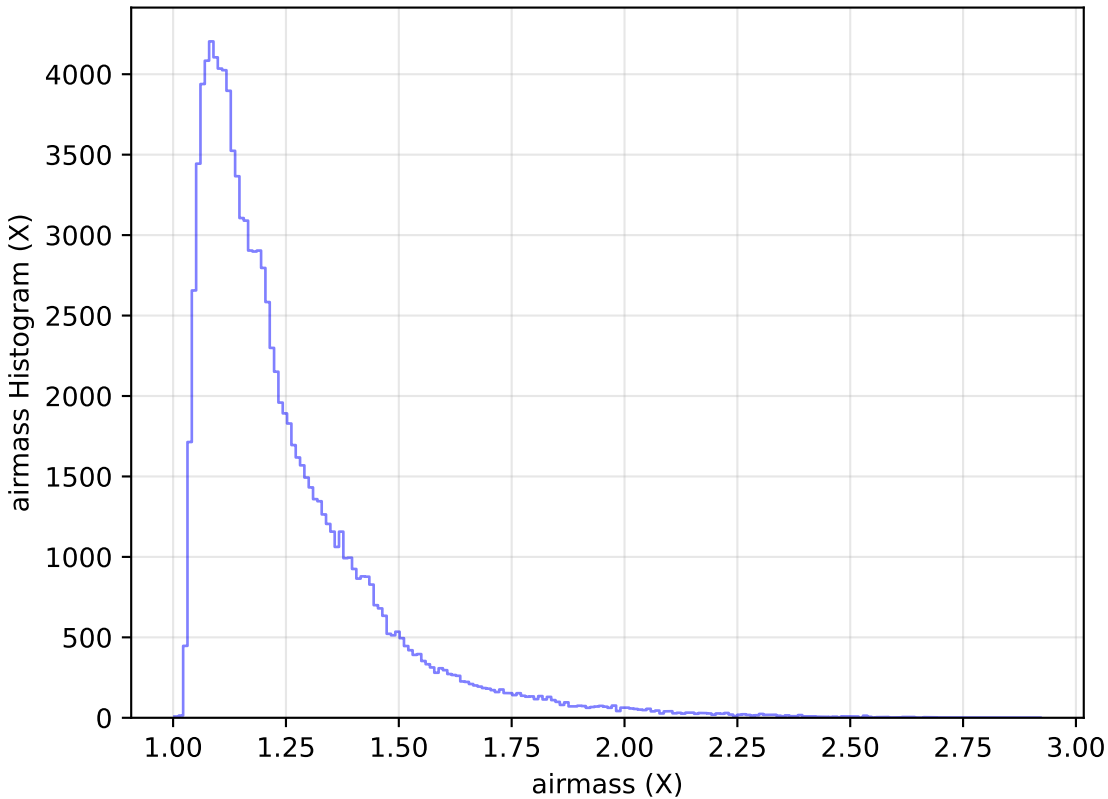
internal_u_expt38_nscale0.9v3.4_10yrs All sky u band: airmass Histogram
