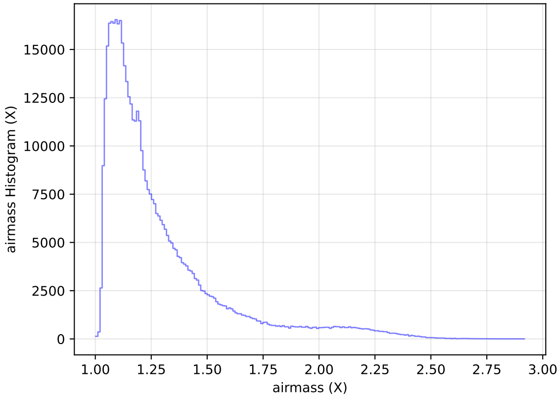
internal_u_expt38_nscale0.9v3.4_10yrs All sky r band: airmass Histogram
